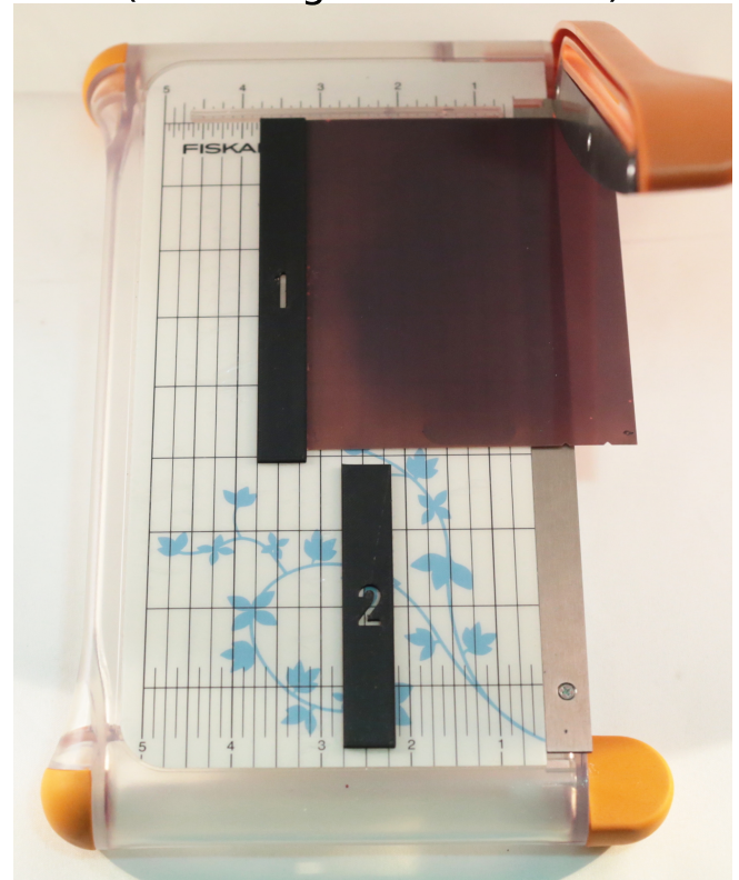
Cutting 4x5 film: Step 1 (trim long side of sheet)
