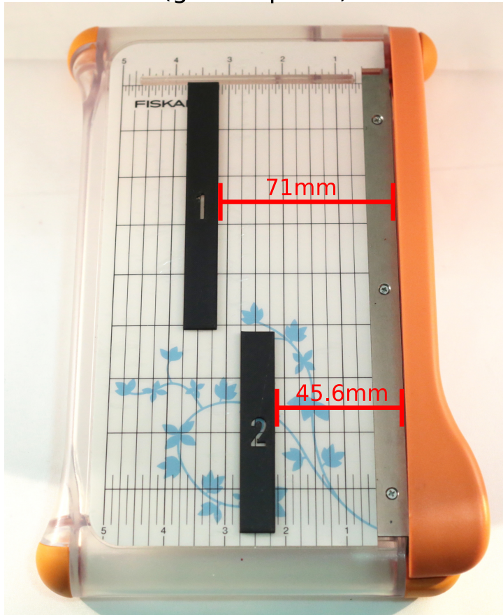
Proper positions of guides (glue in place)
